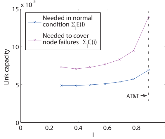
Figure 15. Link capacity
