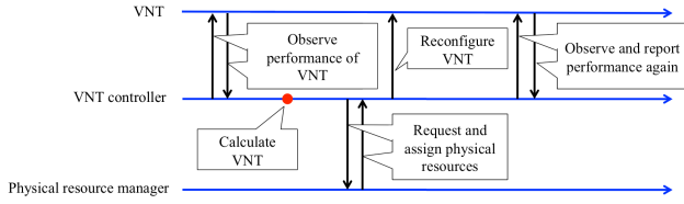
Figure 3. Information exchange for single VNT control
