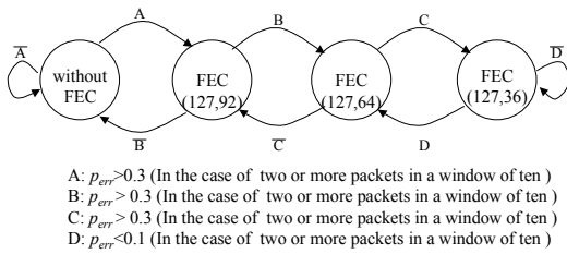
Figure4 Snoop+ELN over Adaptive FEC
