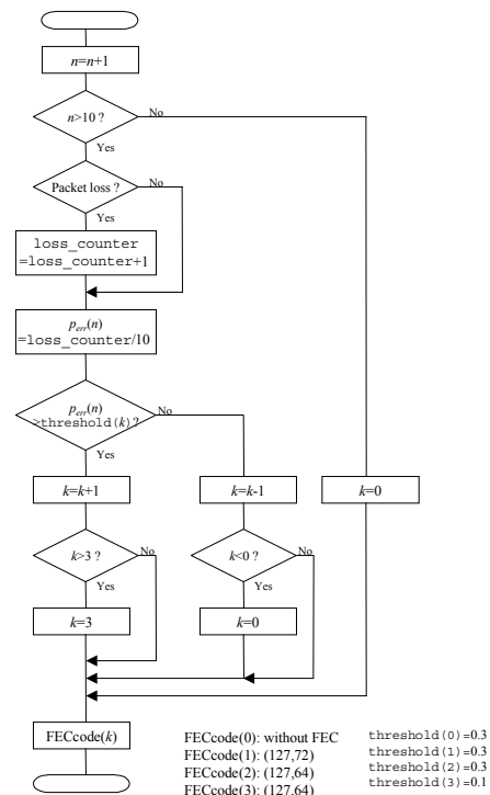
Figure6 Adaptive FEC flow
