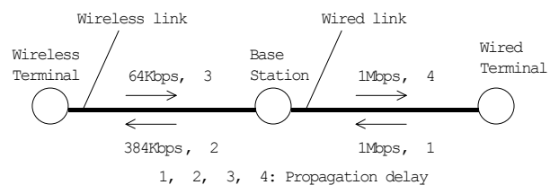
Figure 1 Network model
