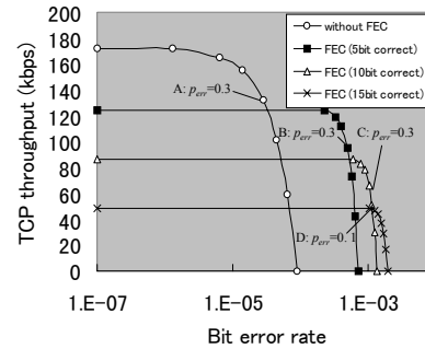
Figure3 Adaptive FEC.
