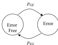
Figure5 Gilbert model
