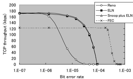
Figure2 TCP throughput
