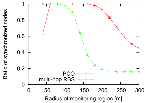
Figure 3 The evaluation over the size of the monitoring region
