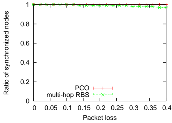
Figure 4 Packet loss performance
