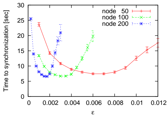
(b) Optimal value of \epsilon for synchronization
