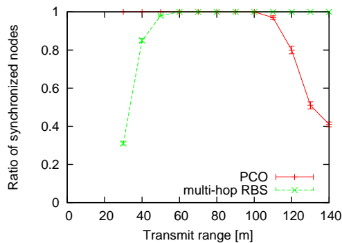
Figure 5 Effective transmit range is different between PCO and multi-hop RBS
